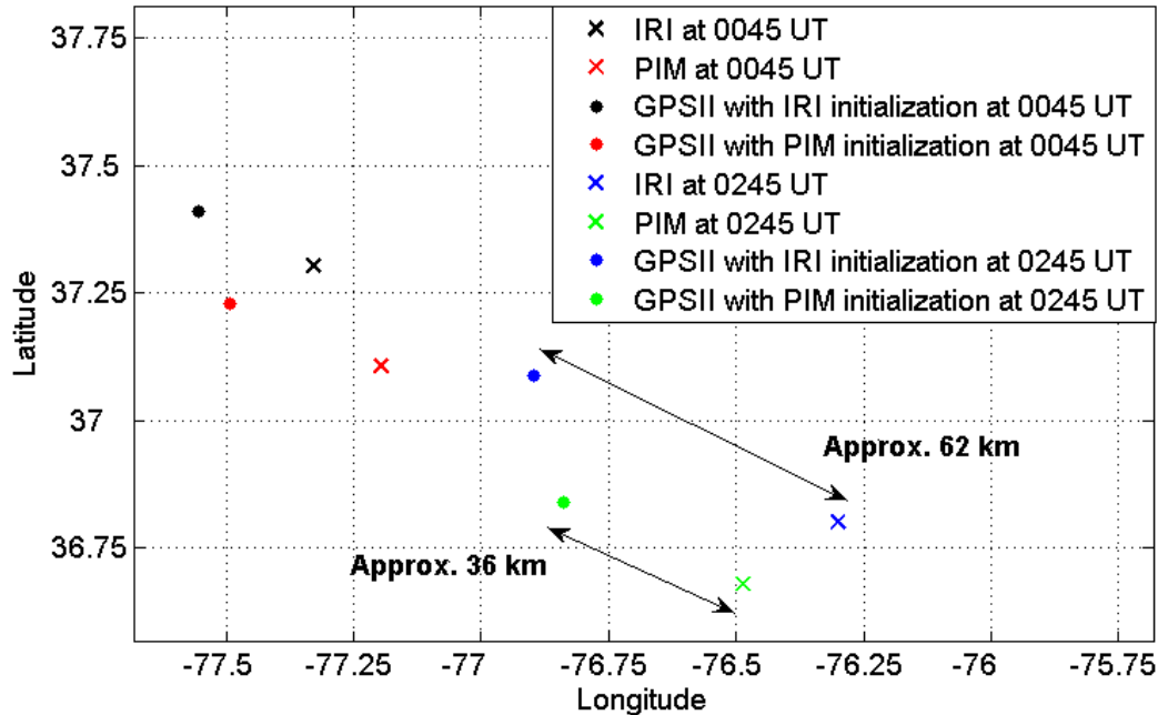
Figure 33: Receiver location (where a signal returns to the Earth's surface) for a 5 MHz signal transmitted from Wright-Patterson AFB, OH toward Norfolk, VA for both the initial positive phase (0045 UT) and main negative phase (0245 UT) of a geomagnetic storm on 27 Aug 98 using various ionospheric models.
