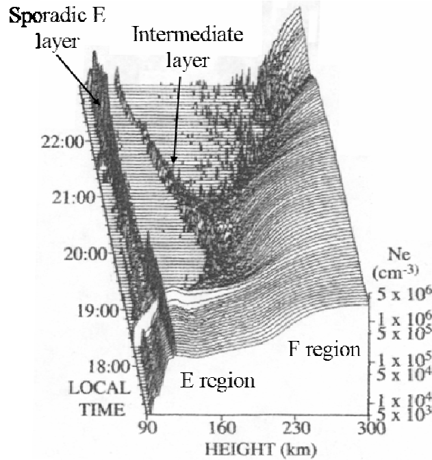
Figure 6: Ionospheric irregular variations. Electron density is shown as a function of both height and time. A sporadic E layer persists for the entire time period, while an intermediate layer begins to descend in height at approx 2000 LT. Density measured with Arecibo incoherent scatter radar on 7 May 1983. [Schunk and Nagy, 2000]
