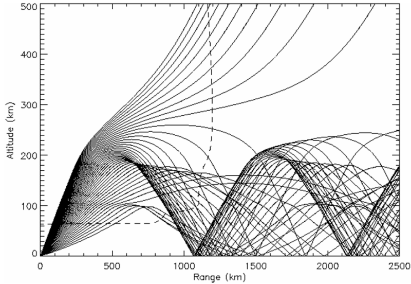
Figure 11: Dependency of signal propagation path on elevation angle. 12.45 MHz signal transmitted with elevation angles increasing from 5^{\circ} – 50^{\circ} (measured from horizon). Dashed line specifies the ionospheric density profile. Notice that the “reflection” altitude (apogee height) increases and the “first hop” ground range initially decreases then ultimately increases with larger elevation angles. [Doherty, 2004]
