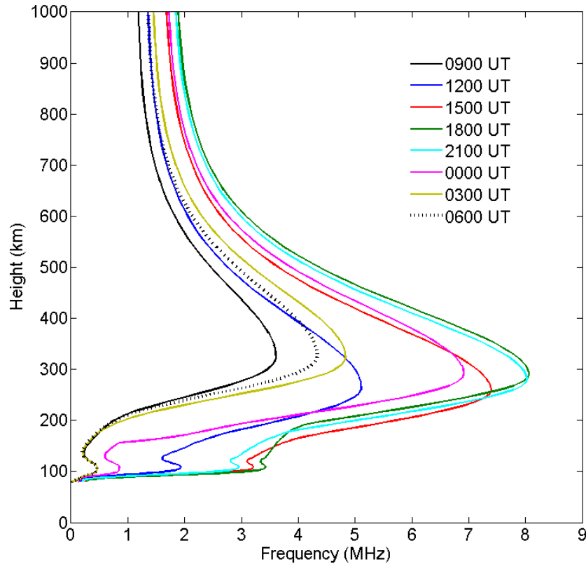
Figure 3: An example of the ionosphere’s diurnal variation. Plasma frequency (MHz) as a function of height (km) at Wright-Patterson AFB on the autumnal equinox during normal solar and geomagnetic activity.
