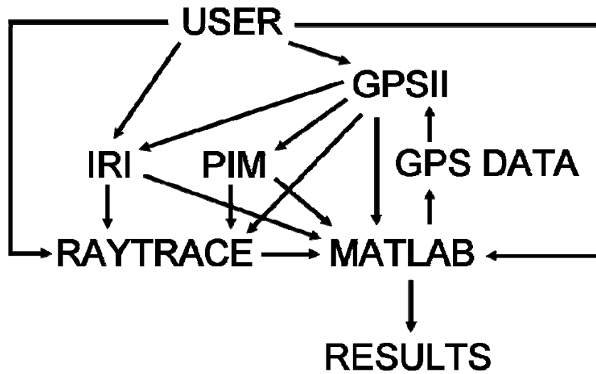
Figure 16: Summary of the flow of data between the user and the required components. The user directs the components to read initialization parameters, process data, and output results in proper formats for visualization and comparison.
