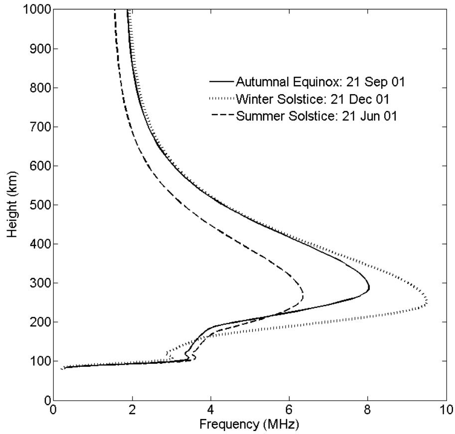
Figure 4: An example of the ionosphere's seasonal variation. Plasma frequency (MHz) as a function of height (km) for Wright-Patterson AFB at local noon on the autumnal equinox and solstices during normal solar and geomagnetic activity.
