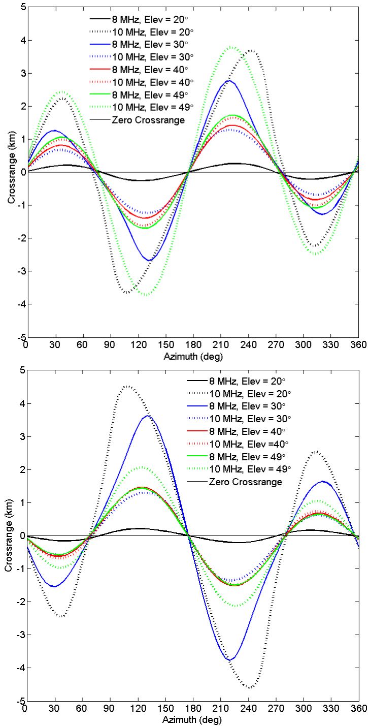
Figure 35: Final crossrange (at the point where the signal returns to Earth, in km) as a function of azimuth angle (deg) for HF signals of various frequencies and elevation angles transmitted from Wright-Patterson AFB at local noon on the autumnal equinox during normal solar and geomagnetic activity. Both the ordinary mode (top) and extraordinary mode (bottom) have zero final crossrange near the four magnetic cardinal points. Final crossrange of ordinary mode is opposite in direction to that of the extraordinary mode for all transmission azimuths.
