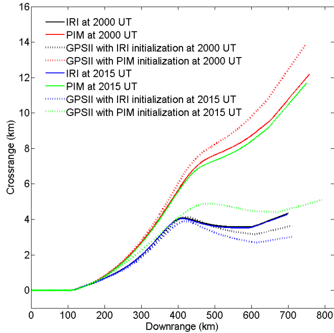
Figure 40: Crossrange (km) as a function of distance downrange (km) for an 8 MHz signal transmitted with elevation = 40.260^\circ from Wright-Patterson AFB, OH toward Norfolk, VA both before (2000 UT) and during (2015 UT) a solar flare on 15 Jul 02 using various ionospheric models.
