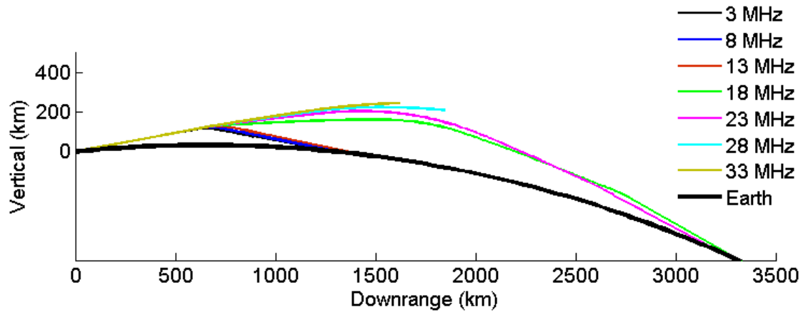
Figure 10: Dependency of signal propagation path on signal frequency. Greater electron densities are needed for higher frequencies to refract. The signal path length increases when refraction occurs later in the propagation. Higher frequencies eventually penetrate the ionosphere. Note that this assumes a horizontally homogeneous ionosphere.
