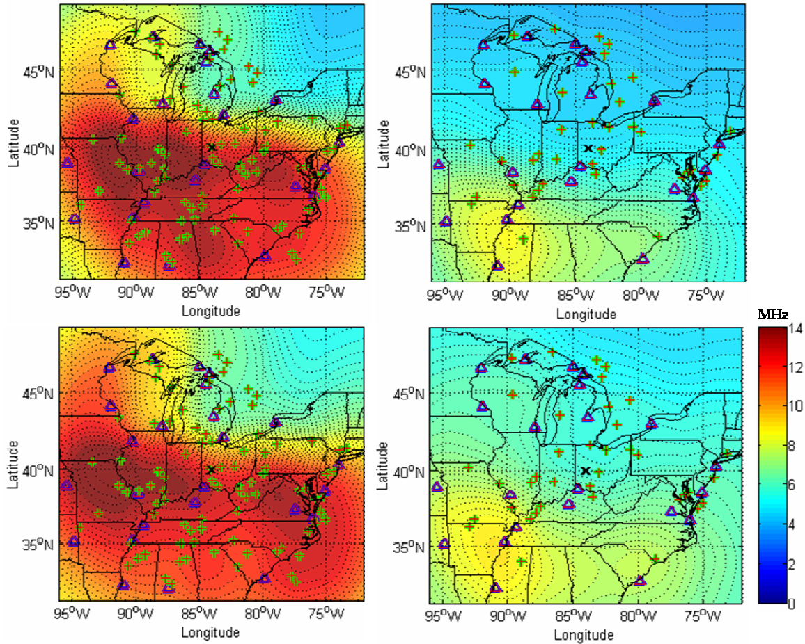
Figure 30: Critical frequency contours (MHz) during a geomagnetic storm on 27 Aug 98. Left column is during the initial positive phase (0045 UT). Right column is during the beginning of the main negative phase (0245 UT). Top row is the GPSII model initialized with the IRI-2001 model. Bottom row is the GPSII model initialized with PIM. Triangles indicate position of GPS ground receivers and crosses show position of ionospheric pierce points (at 400 km) for each satellite-receiver path.
