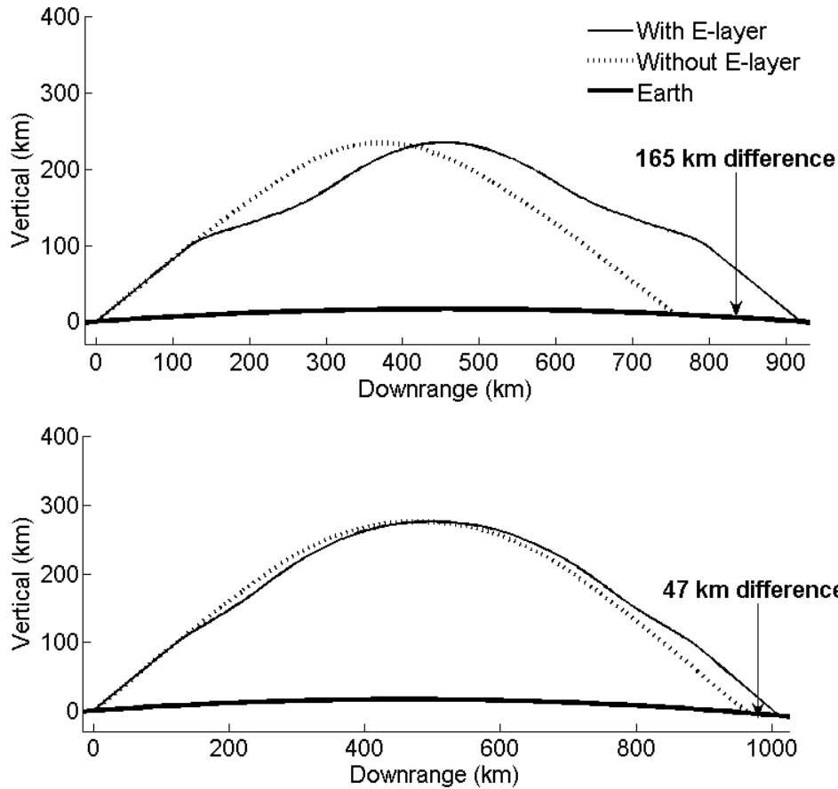
Figure 18: Effect of E layer on signal propagation for two different frequencies. Signals are transmitted with elevation = 35^\circ and azimuth = 180^\circ from Wright-Patterson AFB, OH at local noon on the autumnal equinox during fictitious solar and geomagnetic conditions. Their propagation paths are shown projected onto the x-z plane. Top trajectory is for a 6 MHz signal; bottom trajectory is for an 8 MHz signal. Presence of E layer increases the signals' propagation path (signals return to Earth further downrange). This effect is dramatically less for the slightly higher signal frequency.
