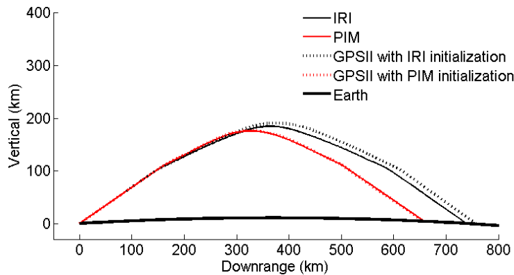
Figure 21: Propagation path projected onto the x-z plane for a 7 MHz signal transmitted from Wright-Patterson AFB, OH toward Norfolk, VA at local noon on 9 Jan 06 (quiet solar and geomagnetic conditions) using various ionospheric models.
