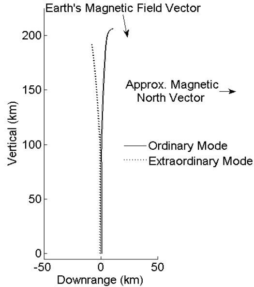
Figure 12: Magnetoionic splitting of a 5 Hz signal transmitted toward zenith from Wright-Patterson AFB at local noon on the autumnal equinox during normal solar and geomagnetic activity. The signal's propagation is affected by the local magnetic field. The signal's ordinary mode refracts to become perpendicular to the local magnetic field vector, while its extraordinary mode refracts to become parallel.
