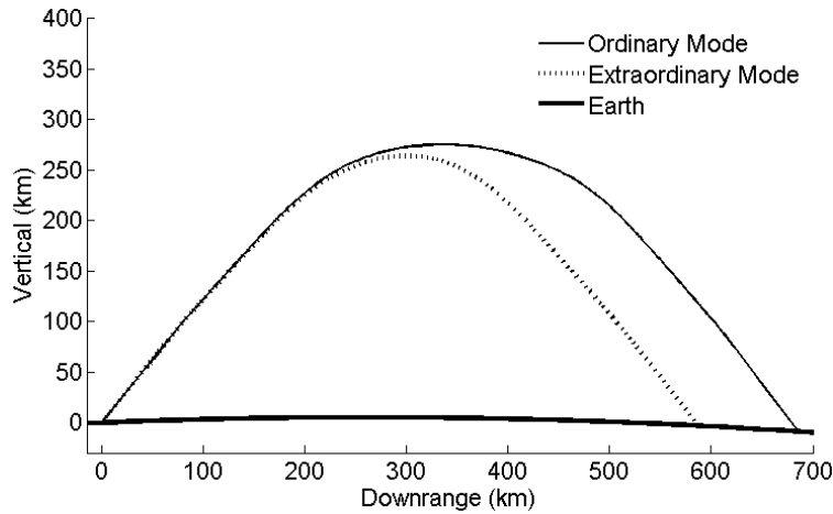
Figure 36: Magnetoionic splitting of a 10 MHz signal transmitted with elevation = 49° and azimuth = 225° from Wright-Patterson AFB at local noon on the autumnal equinox during normal solar and geomagnetic activity. Fundamentally, signal “reflection” occurs when refractive index = 0, thus for ordinary mode when \frac{\omega_{plasma}^2}{\omega_{signal}^2} = 1 and for extraordinary mode when \frac{\omega_{plasma}^2}{\omega_{signal}^2} = 1 - \frac{\omega_{cyclotron}}{\omega_{signal}} . As a consequence, the extraordinary mode “reflects” earlier in its propagation, resulting in a lower apogee height and shorter ground range.
