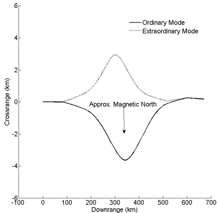
Figure 13: Magnetoionic splitting of a 10 MHz signal transmitted from Wright-Patterson AFB toward magnetic west at local noon on the autumnal equinox during normal solar and geomagnetic activity. Shown is crossrange (km) as a function of distance downrange (km). The signal's ordinary mode deviates toward magnetic north, while its extraordinary mode deviates toward magnetic south.
