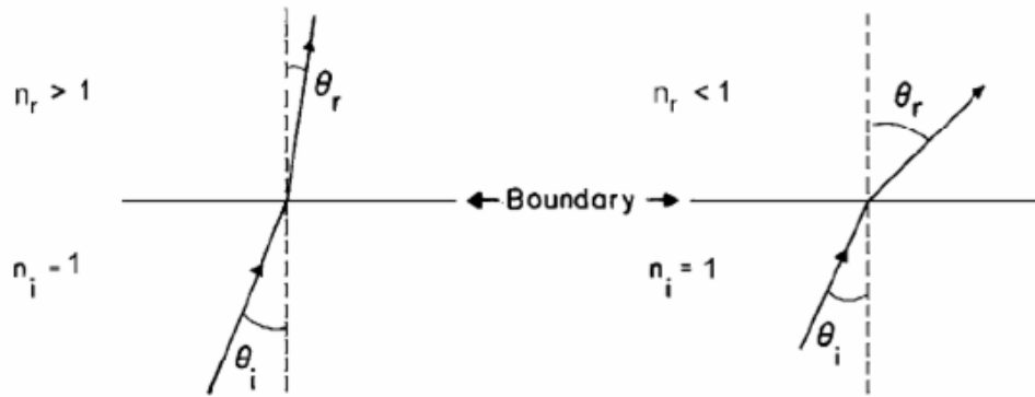
Figure 8: Snell's Law. Electromagnetic wave refracts away from the boundary normal when traveling into medium with smaller refractive index (seen on right side).
