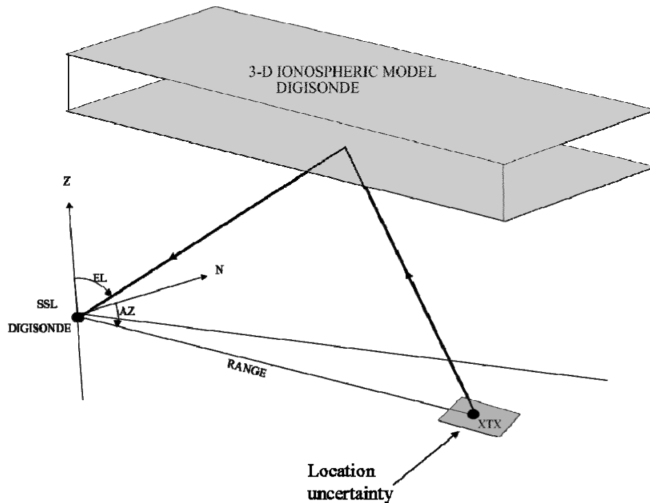
Figure 15: Short-range Single Site Location (SSL) technique using a three-dimensional tilted-slab ionosphere. (DRS Codem Systems, SSL presentation, 2006)
