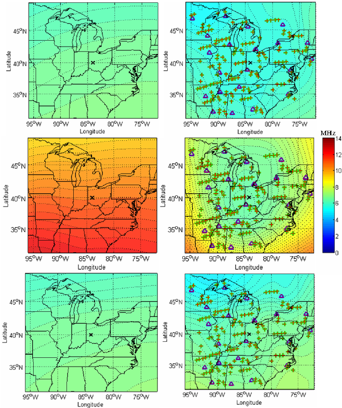
Figure 19: Critical frequency contours (MHz) at local noon on 9 Jan 06 (quiet solar and geomagnetic conditions). Left column is the initialization model. Right column is the GPSII model using the initialization model from the left column. Top row uses IRI-2001 initialization. Middle row uses unphysical initialization conditions compared to the actual quiet conditions of 9 Jan 06, showing how the GPSII model adjusts for unphysical initialization. Bottom row uses PIM initialization. Triangles indicate position of GPS ground receivers and crosses show position of ionospheric pierce points (at 400 km) for each satellite-receiver path.
