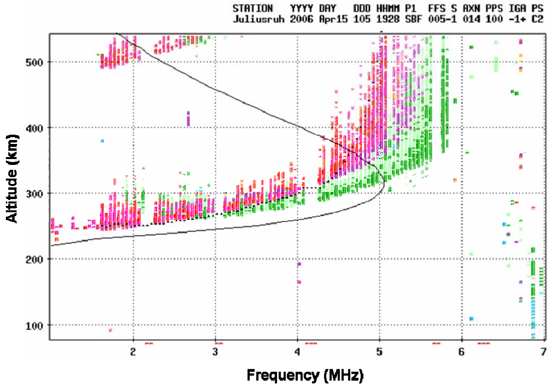
Figure 2: A real-time ionogram created from a vertical incident ionosonde in Juliusruh on 15 April 2006 by the Leibniz-Institute of Atmospheric Physics. The transmitter emits a sweep of frequencies, the receiver detects the refracted signals, and then a “virtual height of reflection” is calculated from the signals’ travel time. The black line is the electron density profile computed from the virtual height. Colors denote strength of signal return (warm colors = stronger dB). The ionosphere above the F 2 peak cannot be measured from a vertical sounding, thus models are used to estimate this.
