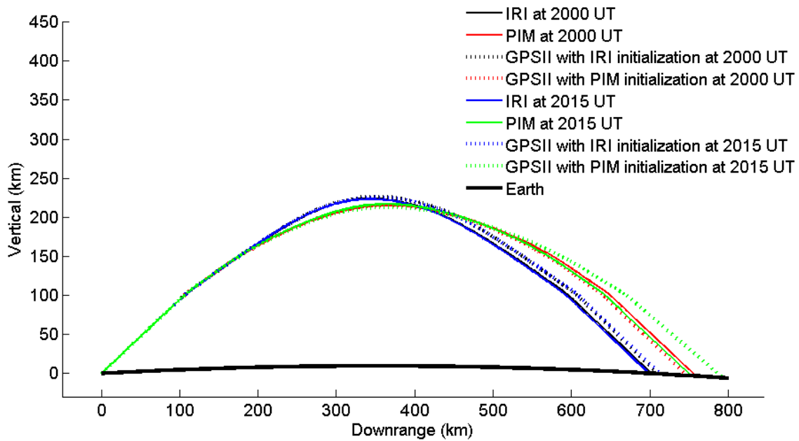
Figure 28: Propagation path projected onto the x-z plane for an 8 MHz signal transmitted from Wright-Patterson AFB, OH toward Norfolk, VA both before (2000 UT) and during (2015 UT) an X3 solar flare on 15 Jul 02 using various ionospheric models.
