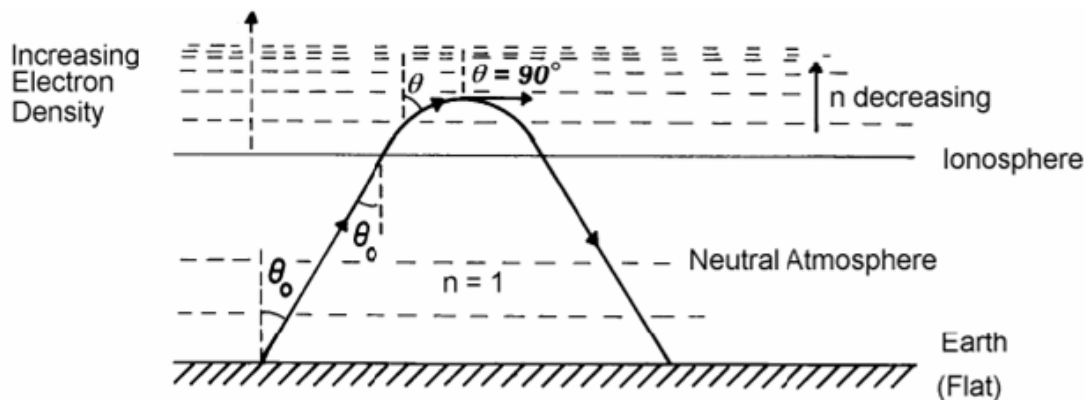
Figure 9: Application of Snell's Law in the ionosphere. The electromagnetic signal progressively refracts away from the boundary normal until the signal propagates perpendicular to the normal. Signal must be treated as a wave to account for continued refraction. Notice that the refractive index decreases with altitude, while the electron density increases with altitude.
