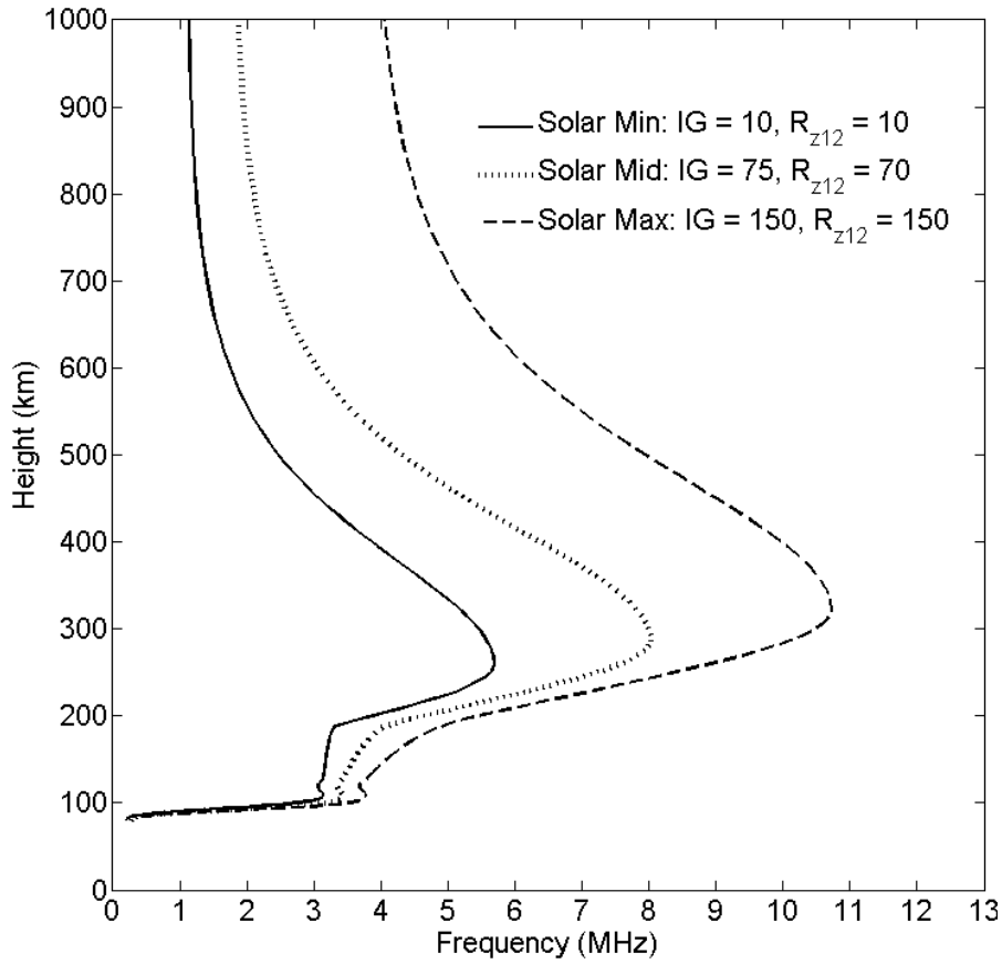
Figure 5: An example of the ionosphere’s solar cycle variation. Plasma frequency (MHz) as a function of height (km) for Wright-Patterson AFB at local noon on the autumnal equinox during normal geomagnetic activity.
