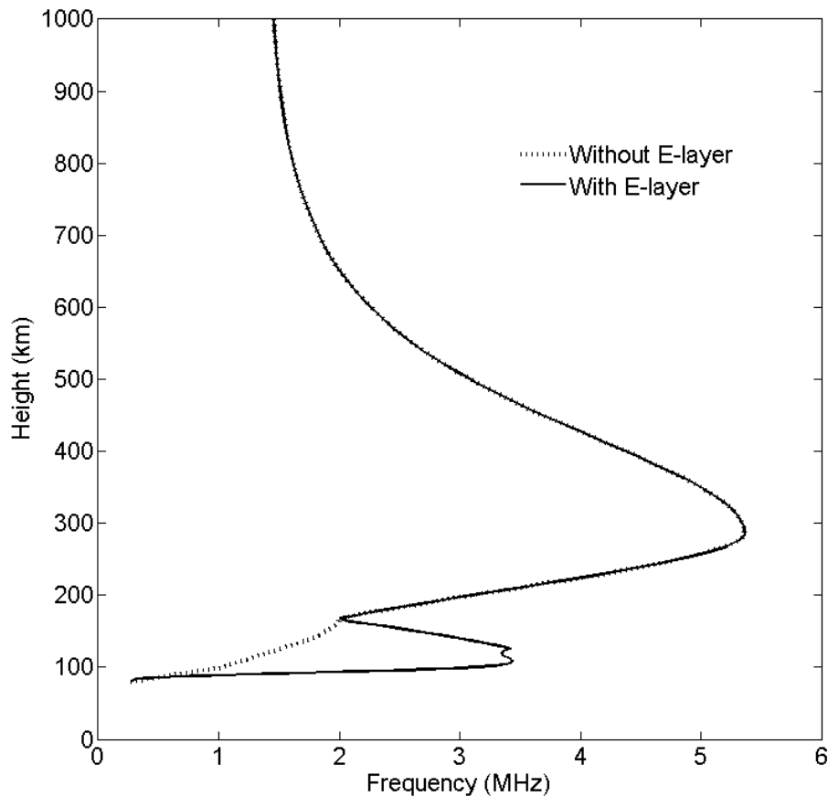
Figure 17: E layer variation. Plasma frequency (MHz) as a function of height (km) for Wright-Patterson AFB at local noon on the autumnal equinox during fictitious solar and geomagnetic conditions.
