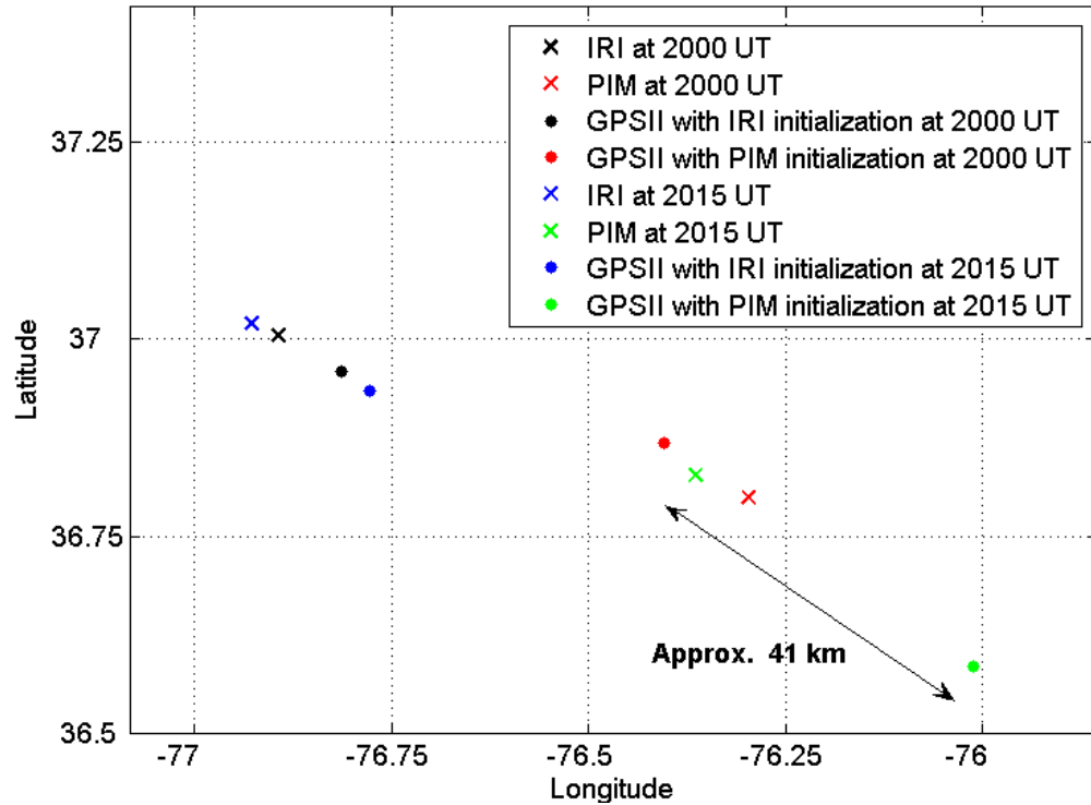
Figure 29: Receiver location (where a signal returns to the Earth's surface) for a signal transmitted from Wright-Patterson AFB, OH toward Norfolk, VA both before (2000 UT) and during (2015 UT) an X3 solar flare on 15 Jul 02 using various ionospheric models.
