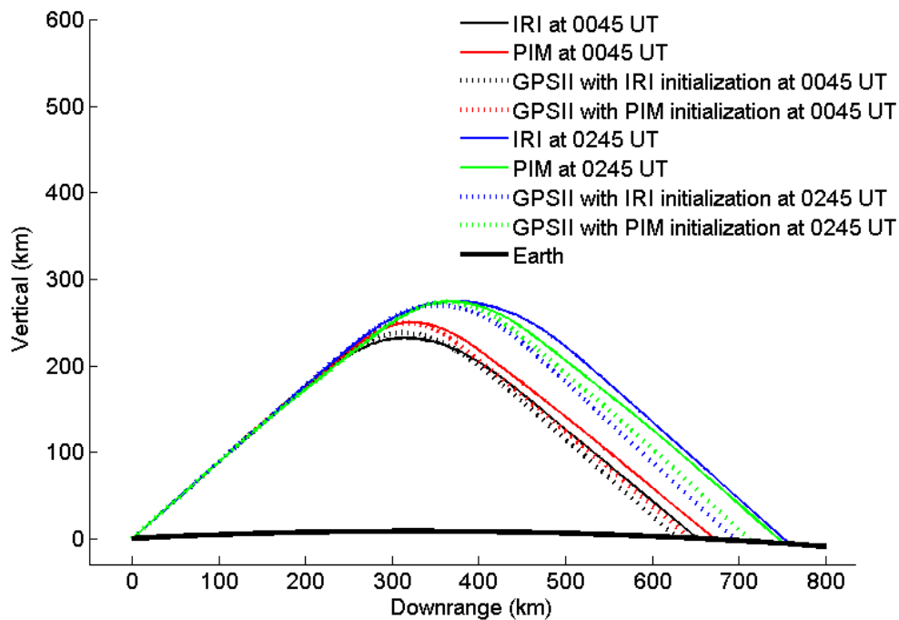
Figure 32: Propagation path projected onto the x-z plane for a 5 MHz signal transmitted from Wright-Patterson AFB, OH toward Norfolk, VA for both the initial positive phase (0045 UT) and main negative phase (0245 UT) of a geomagnetic storm on 27 Aug 98 using various ionospheric models.
